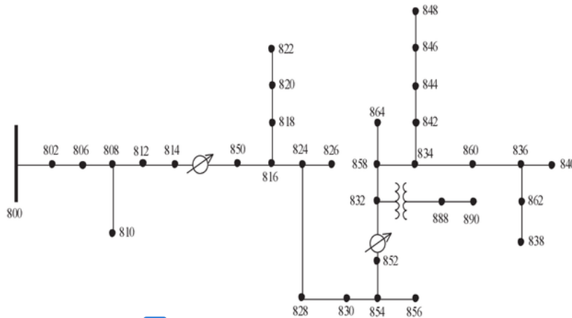
12 FIGURE 2. Single line diagram of a 34-bus radial system
